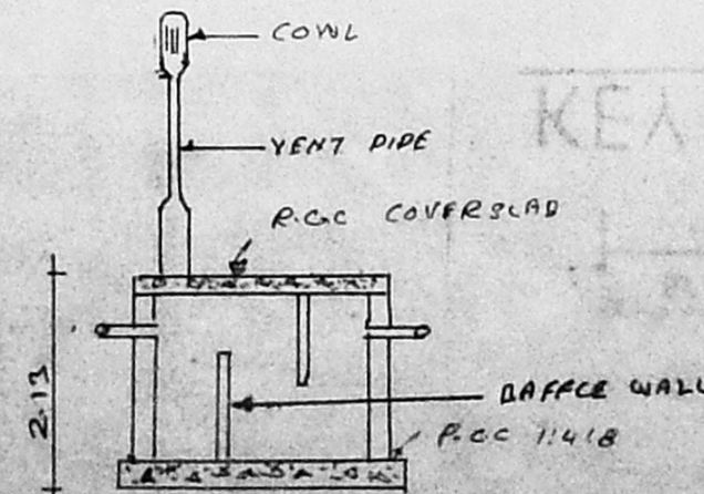
PLAN & SECTION OF SEPTIC TANK
